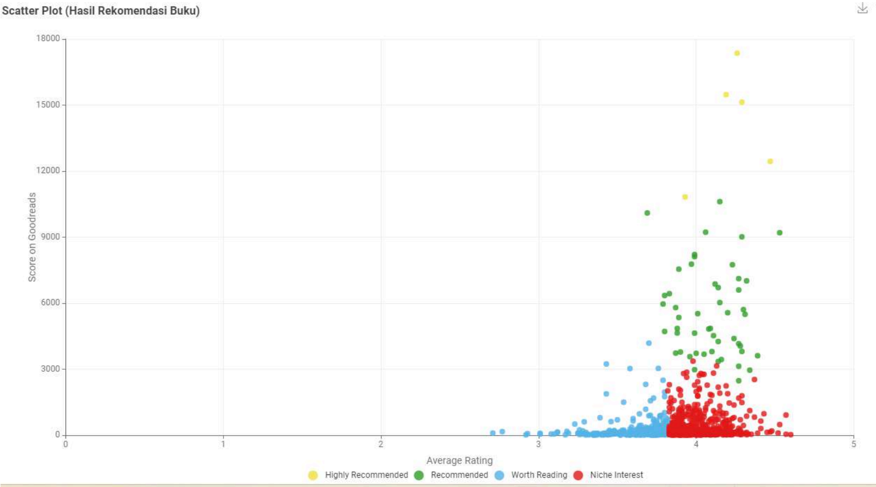
Hasil Average Rating, Score on Goodreads terhadap Cluster
